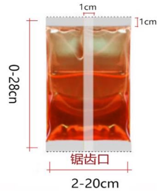
Back seal
